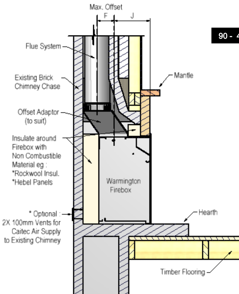
SIDE VIEW OF STANDARD ADAPTOR Note: The maximum offset.
