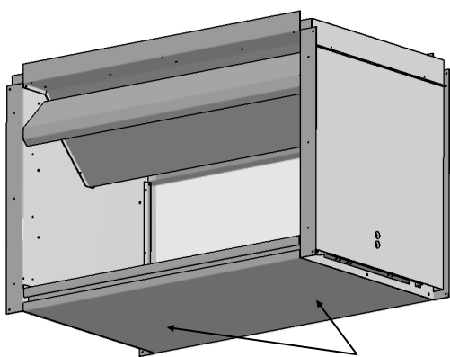
Seismic Restraint Secure Firebox through anchor points provided
