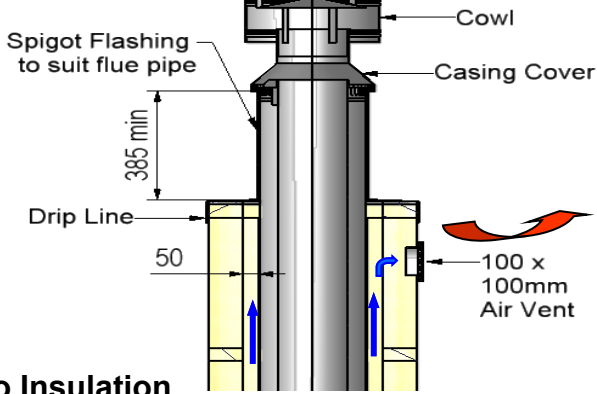
‘No Insulation under flashing’
