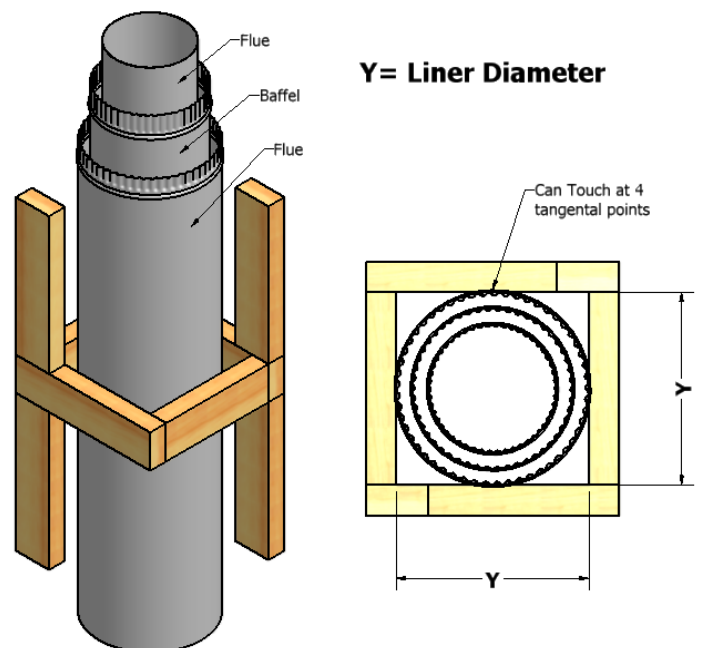
Option Y – Double Lined Flue System
