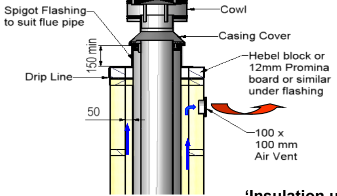
‘Insulation under flashing’
