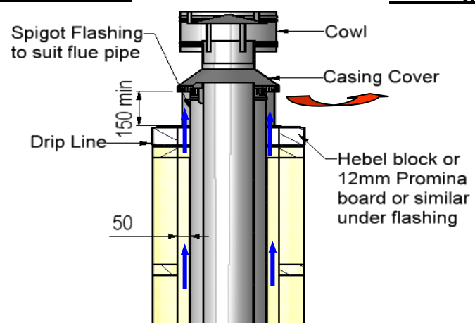
‘Insulation under flashing’
