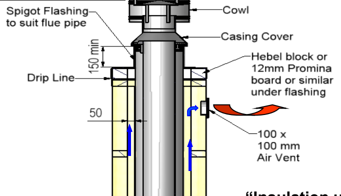
“Insulation under flashing”
