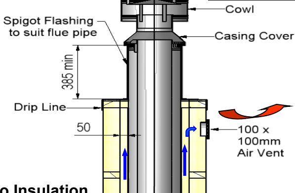
“No Insulation under flashing”
