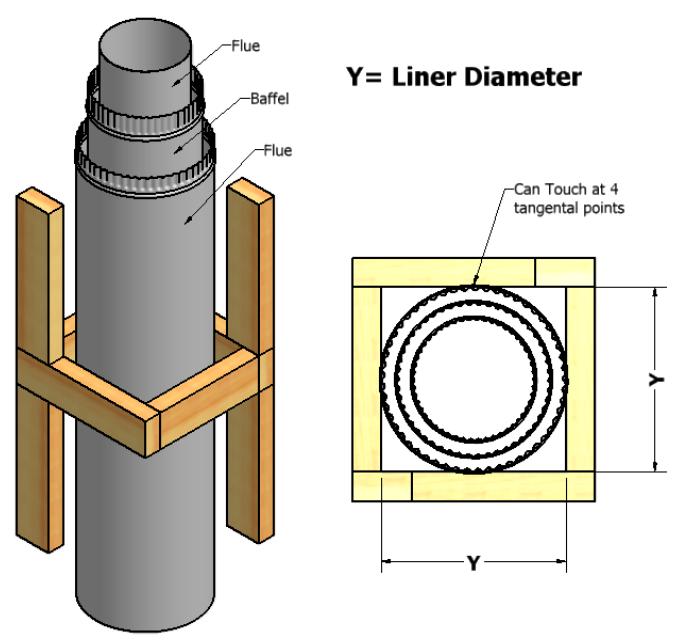
Option Y – Double Lined Flue System
